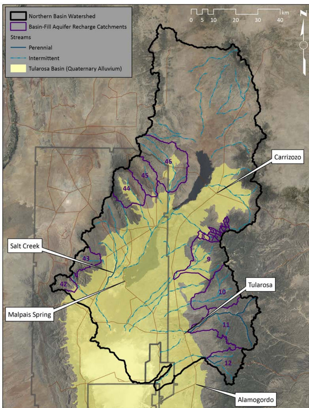
Figure 5. Basin-fill aquifer recharge catchments delineated in the northern Tularosa basin (from Huff, 2005: 6). Catchments are (counterclockwise from north): 46 (Taylor Canyon); 45 (Red Canyon); 44 (Oscura Mountains backslope); 43 (Thurgood Canyon); 42 (Good Fortune and Dry canyons); 12 (Fresnal and La Luz canyons); 11 (Nogal and Tularosa canyons); 10 (Rinconada Canyon); 9 (Three Rivers Canyon); 1-8 (White Mountain Wilderness west-side drainages). Not all catchments are characterized (see Waltemeyer, 2001).
