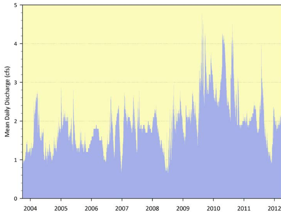
Figure 11. Mean daily discharge at Malpais Spring. Period of record is 1 October 2003 through 4 April 2012 (U.S. Geological Survey, 2014b).
