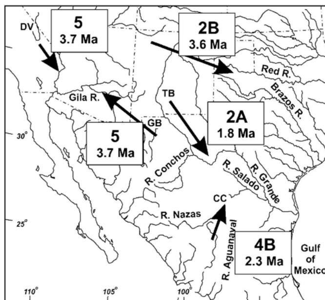
Figure 2. Hypothetical paleosystems and estimated times of vicariance for pupfish in each system. Arrows indicate paleosystems. The Tularosa basin is indicated by TB. Pupfish clades discussed in the text are: 2A = maritime (which includes C. tularosa ); 2B = southern Great Plains-northern Chihuahuan Desert. Figure excerpted from Echelle and others (2005: Figure 4).
