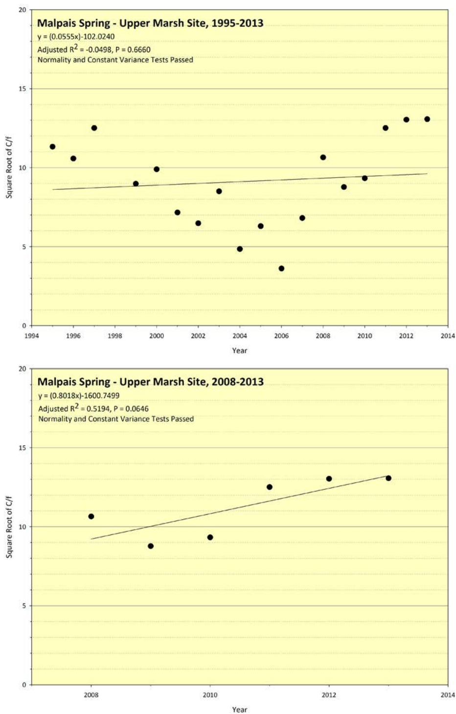
Figure A3. Regression analysis of total C/f at the Upper Marsh site, 1995-2013 (top graph) and 2008-2013 (lower graph).
