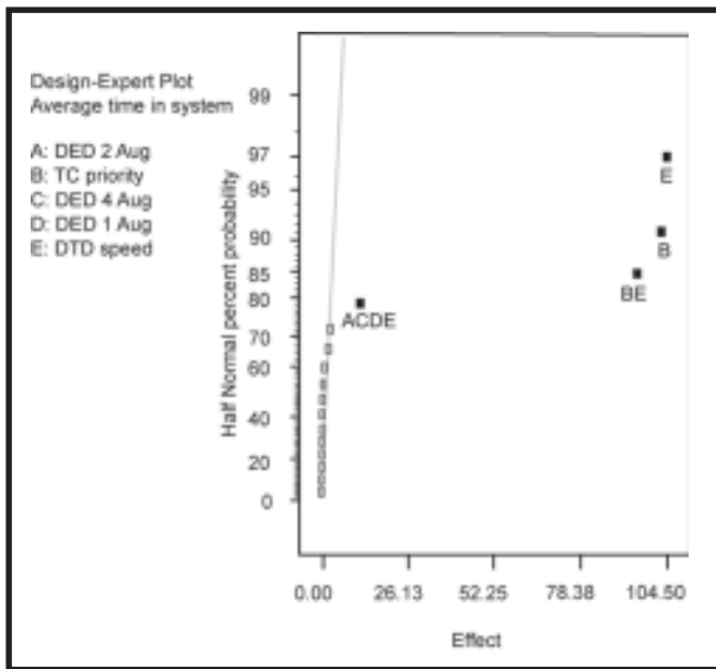
Figure 6. Half normal plot
