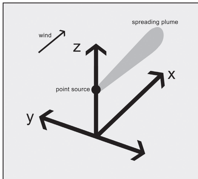
Figure 1. Gaussian distributions
