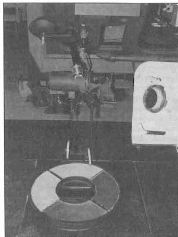
Rear section of FOX with dual sampling wheels and simulated road surfaces.
