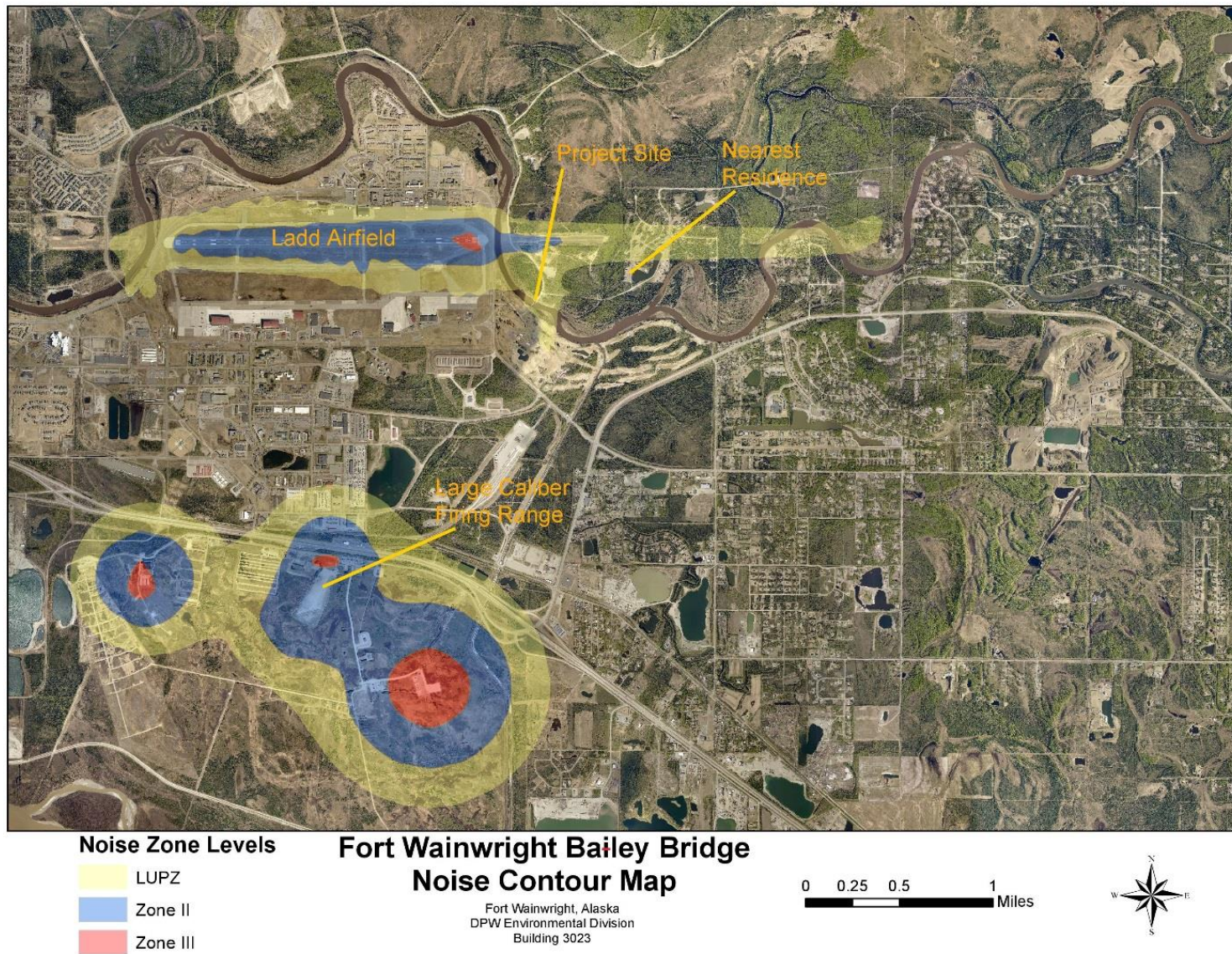
Figure 9. Noise Sources and Sensitive Receptors
