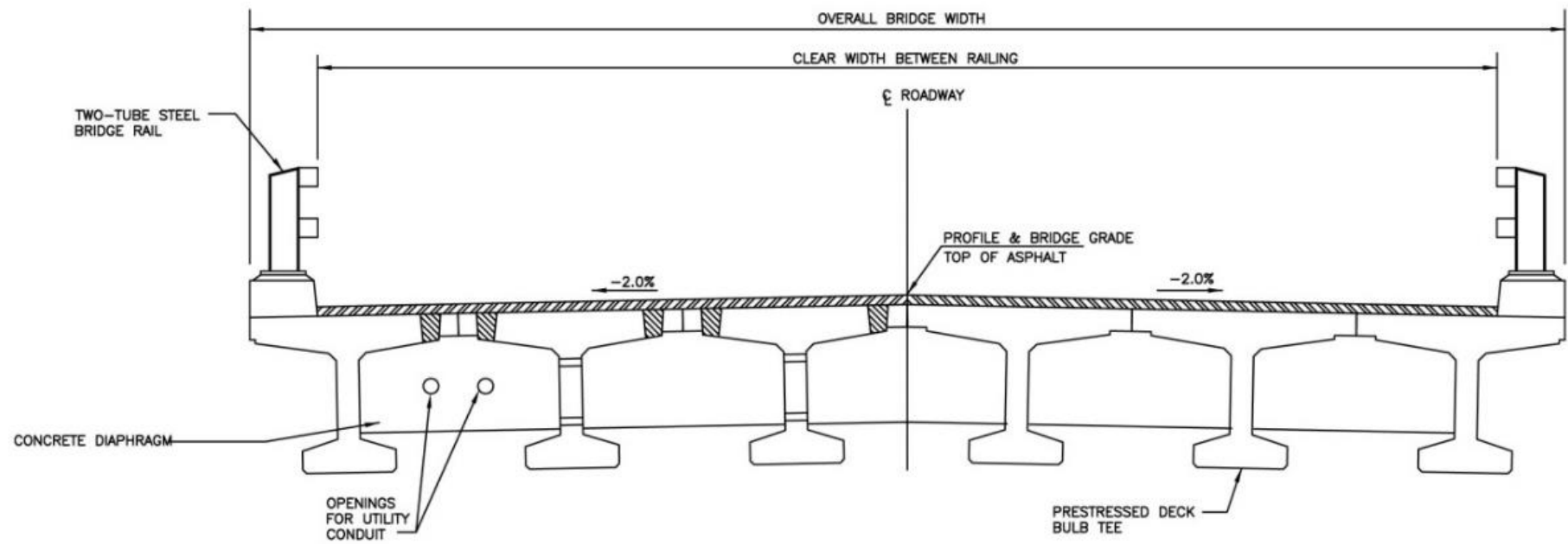
Figure 4. Section Drawing of a Typical Precast-Concrete Bulb-Tee Bridge
