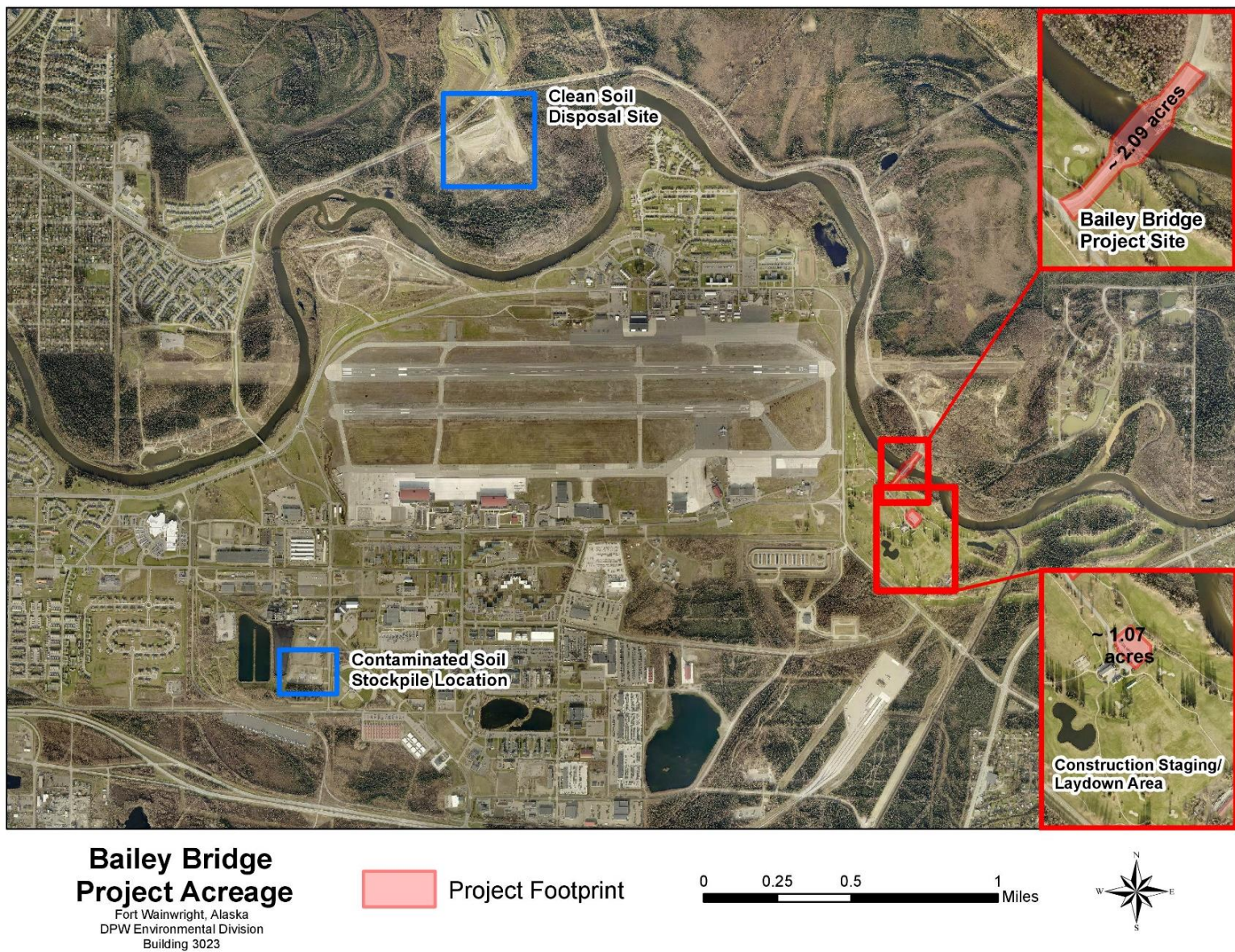
Figure 5. Aerial Photograph Showing Project Area and Anticipated Construction Footprint
