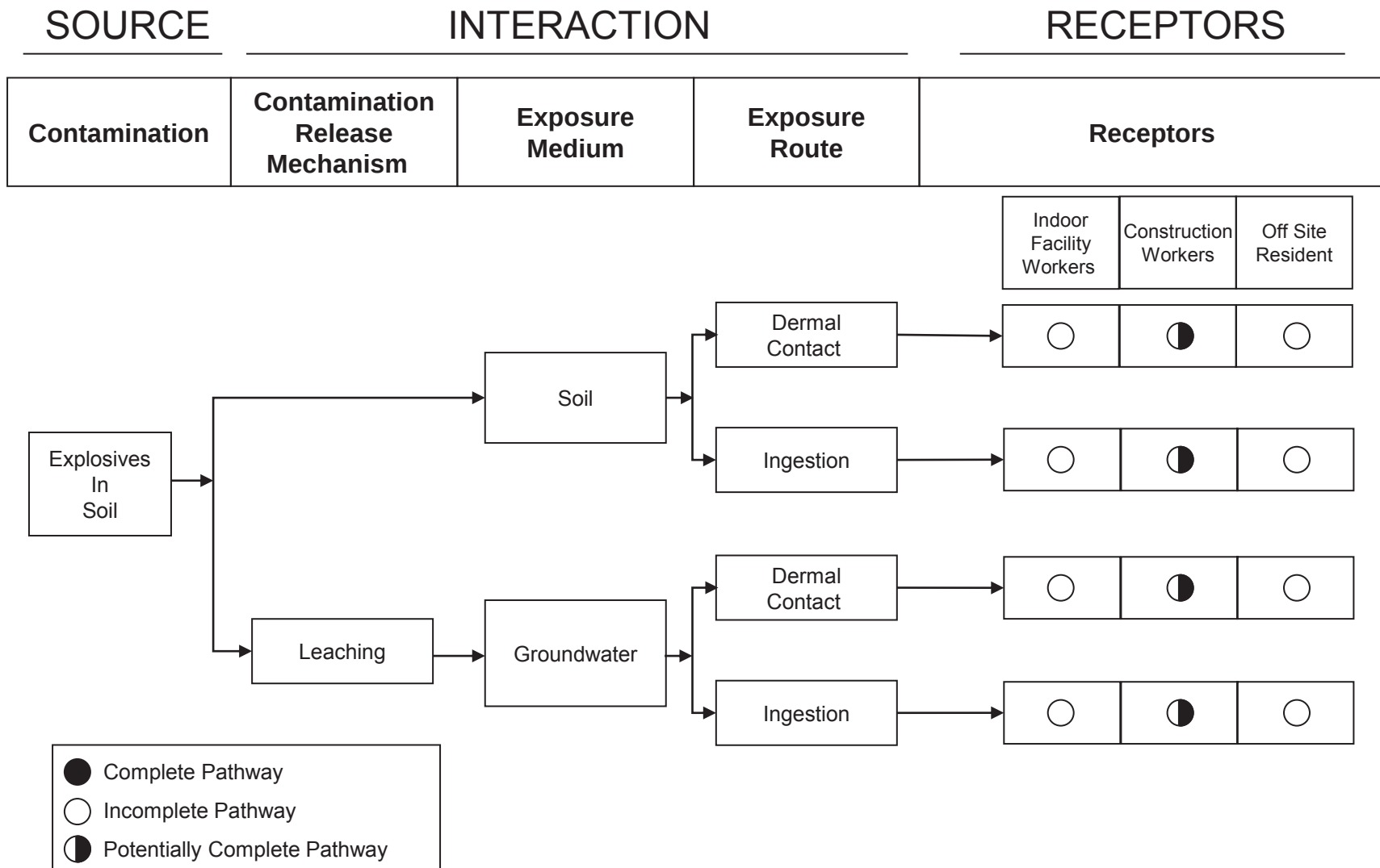
Figure 4-15 MC Conceptual Site Model Grenade Launcher Range
