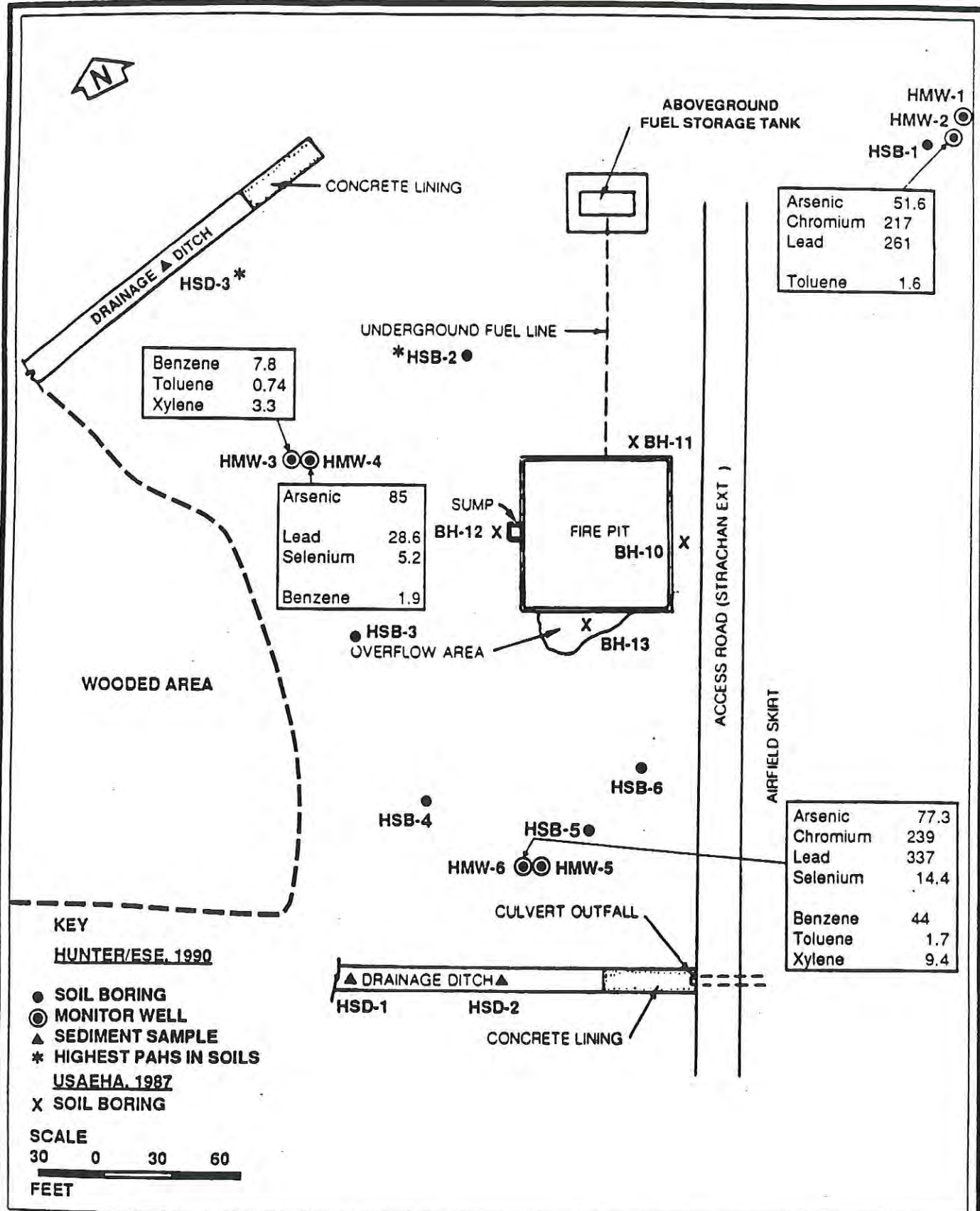
Figure 4-4 CONCENTRATIONS OF METALS (μg/L) ABOVE SDWA AND POTENTIALLY HARMFUL VOCs (μg/L) IN GROUNDWATER AT HUNTER AAF
