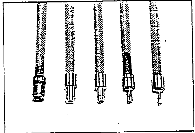
AT-86 Series Wire Screen Implants (left to right, AT-86-SW, AT-86-30S, AT-86-25S, AT-17S, AT-86-12S).
