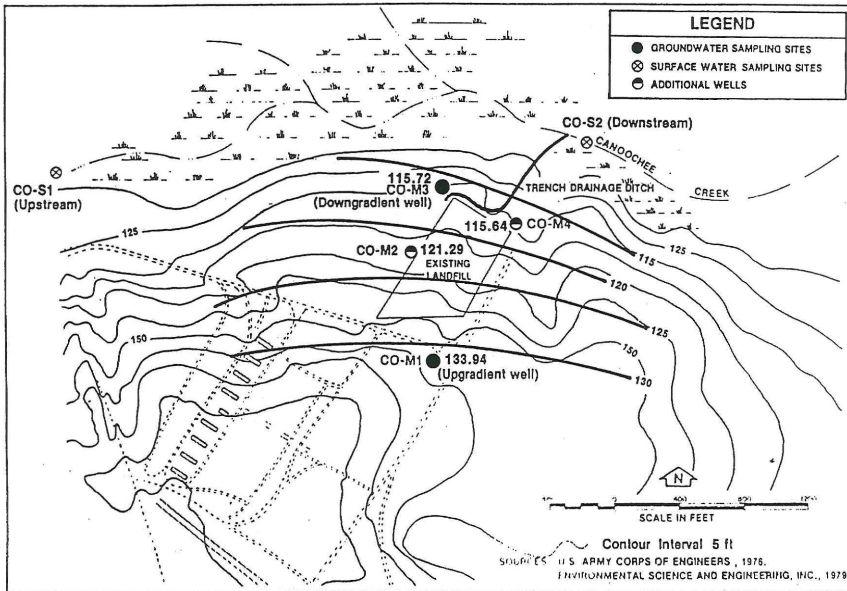
FIGURE D-9. WATER TABLE CONTOUR MAP OF THE CAMP OLIVER LANDFILL AT FORT STEWART, GA.
