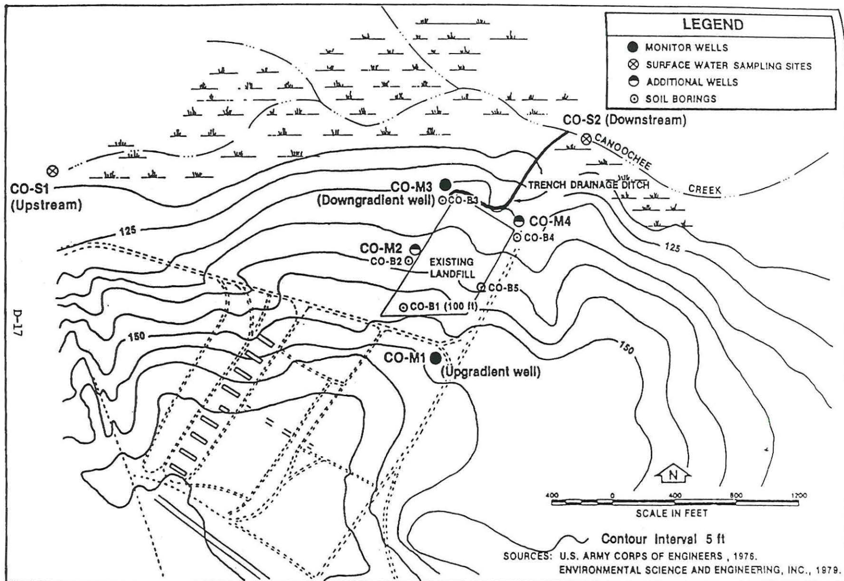
FIGURE D-8. SURFACE ELEVATION CONTOUR MAP OF THE CAMP OLIVER LANDFILL SHOWING LOCATIONS OF TWO GROUND-WATER MONITORING WELLS AND TWO WELLS DRILLED FOR ADDITIONAL WATER LEVEL DATA
