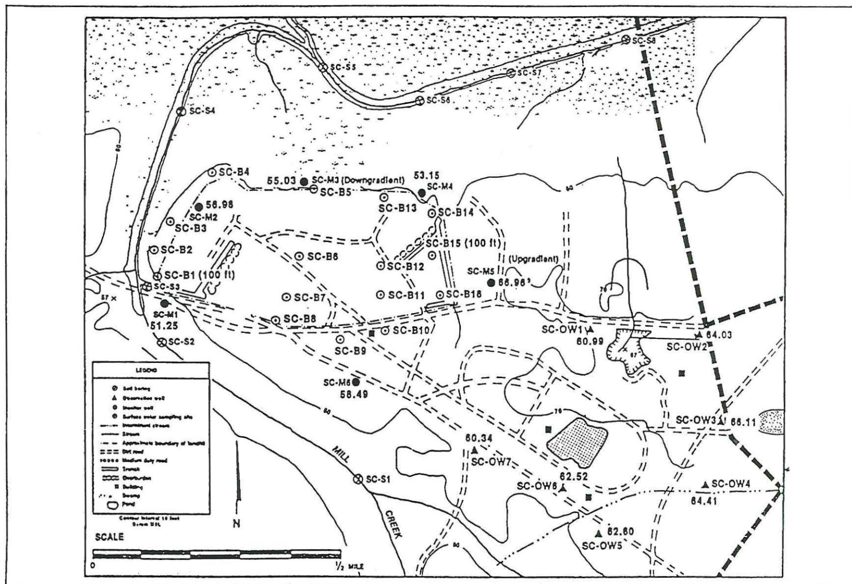
FIGURE D-6. MAP OF SOUTH - CENTRAL LANDFILL SHOWING LOCATIONS OF SIX GROUND-WATER MONITORING WELLS AND SEVEN OBSERVATION WELLS
