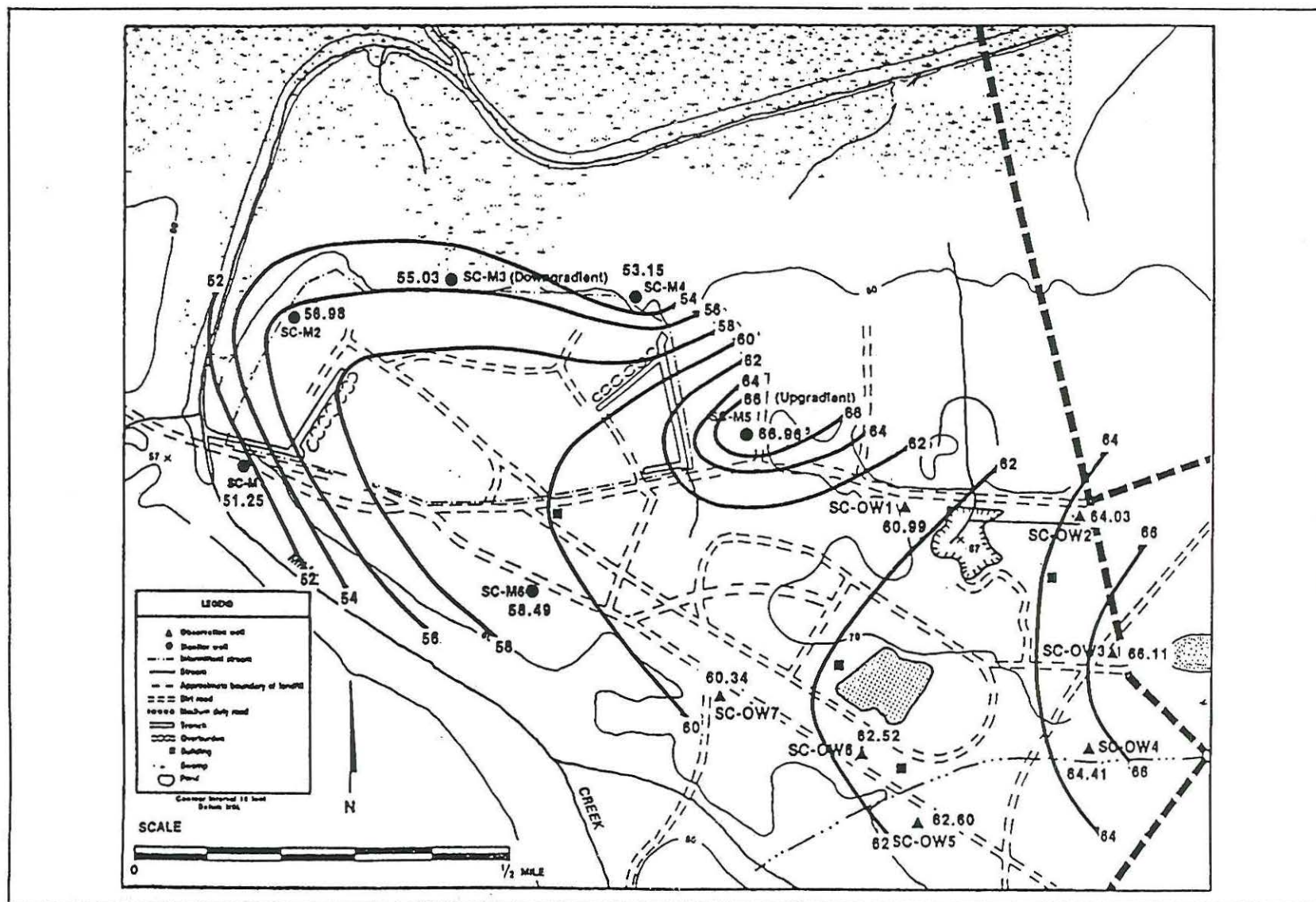
FIGURE D-7. WATER TABLE CONTOUR MAP OF THE SOUTH-CENTRAL LANDFILL AT FORT STEWART, GA.
