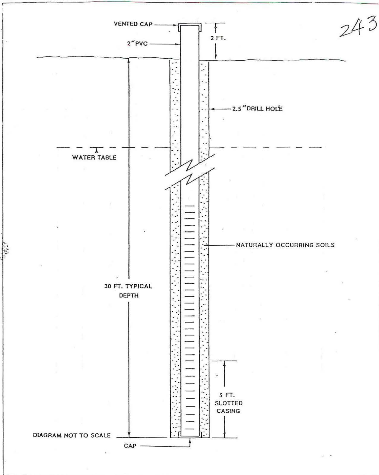
FORT STEWART TYPICAL OBSERVATION WELL INSTALLATION
