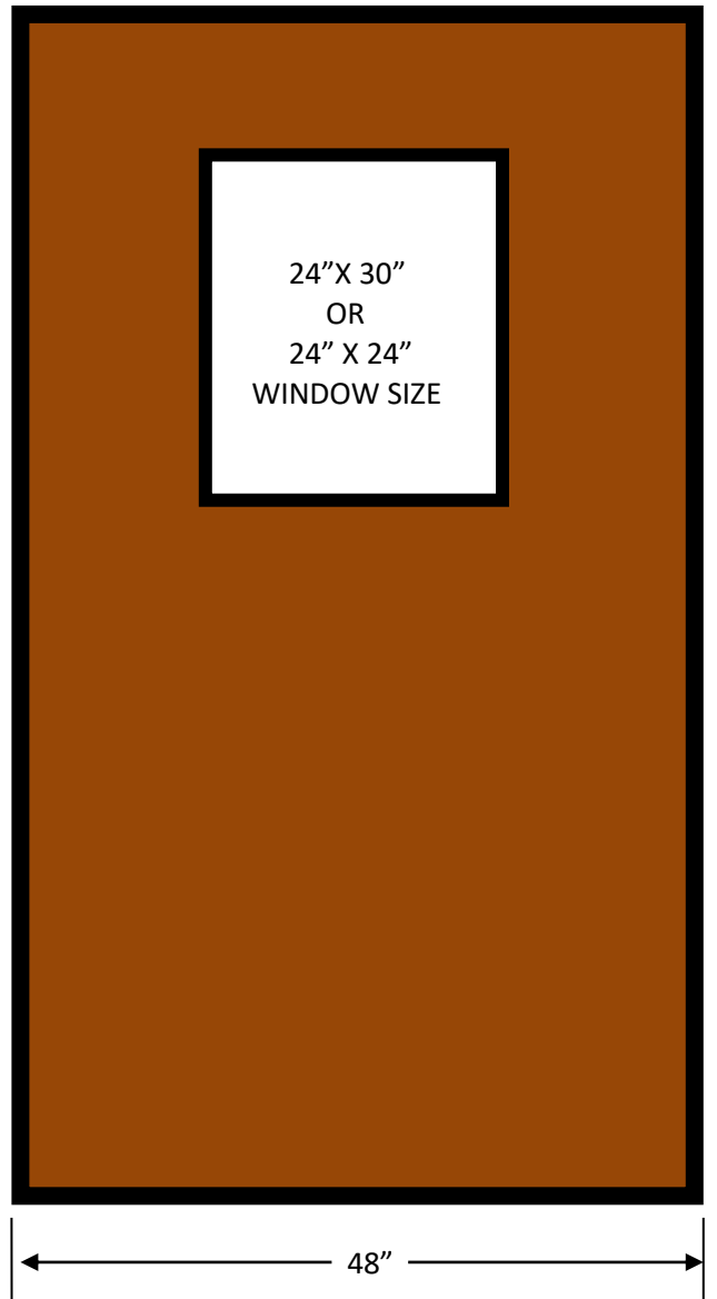
BARRIER, WINDOW FRAME WALL
