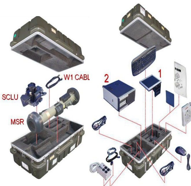
DVC # 07-126 JAVELIN BASIC SKILLS TRAINER (BST)
