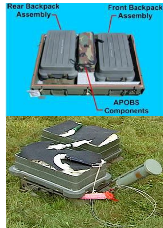
DVC # 05-103/1 ANTI- PERSONNEL OBSTACLE BREACHING SYSTEM (APOBS)
