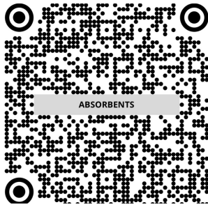
Absorbents
