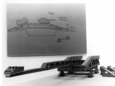
GIRDER BRIDGE MODEL
