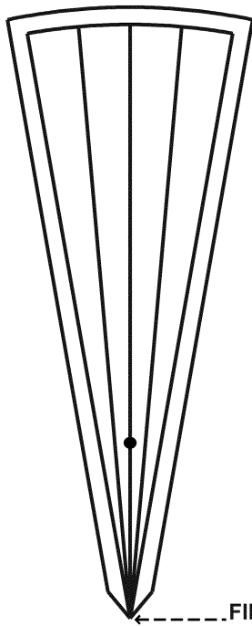
Figure 3-4. Cone surface danger zone for small- arms direct-fire weapons with explosive projectiles
