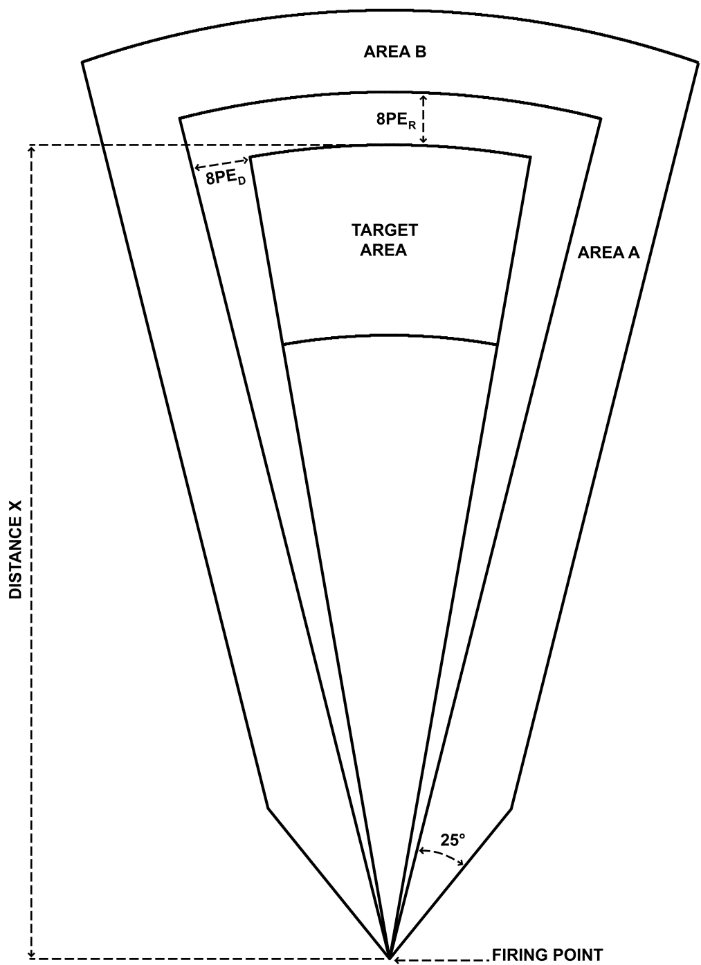
Figure 9-1. Surface danger zone for firing mortars
