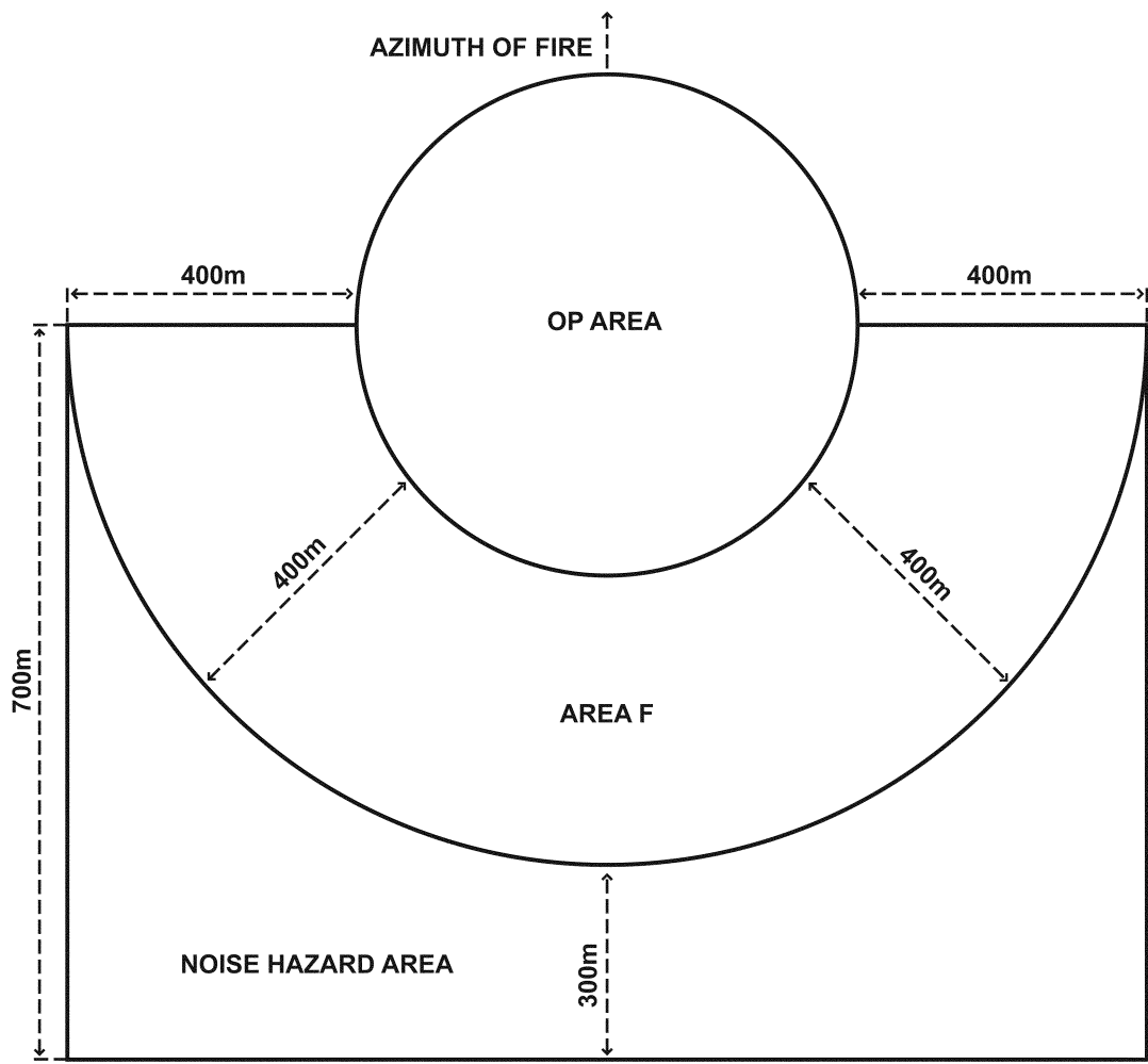
Figure 10-14. Area F for reduced range practice rocket operational area
