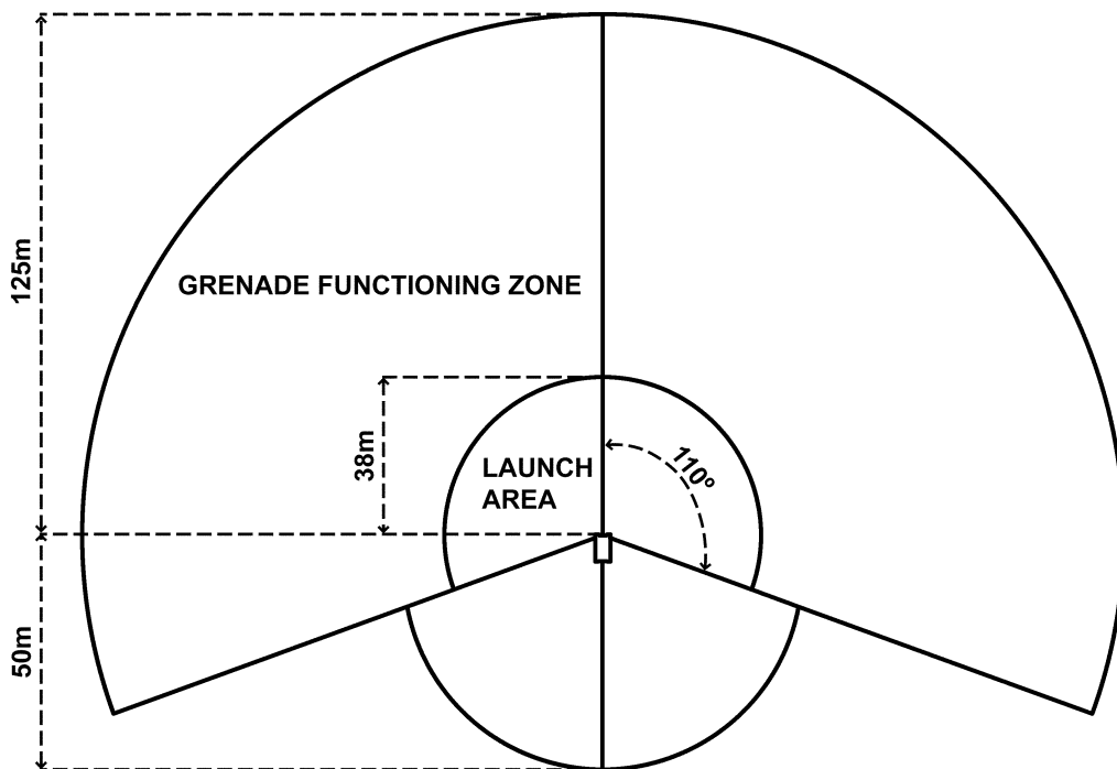
Figure 8-10. Surface danger zones for firing L8A1/A3 smoke grenades
