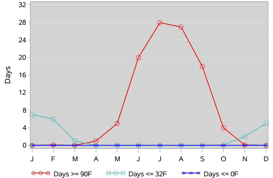
Temperature Days
