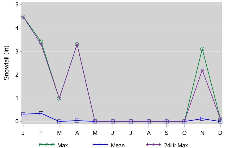
Snowfall
