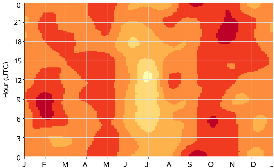
Rain/Drizzle Occurrence
