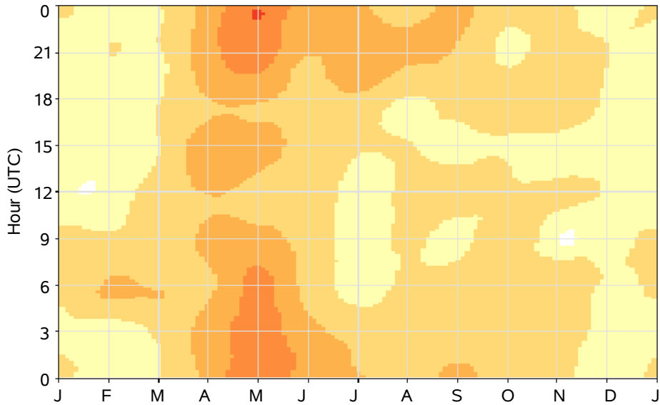
Thunderstorm Occurrence
