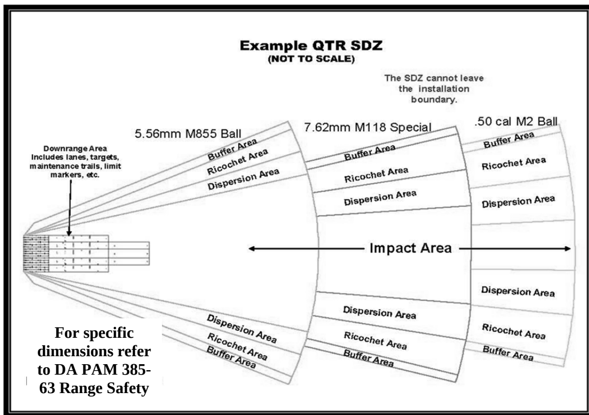
Figure 3. Example of a Surface Danger Zone (SDZ) at a United States Army Qualification Training Range (QTR).
