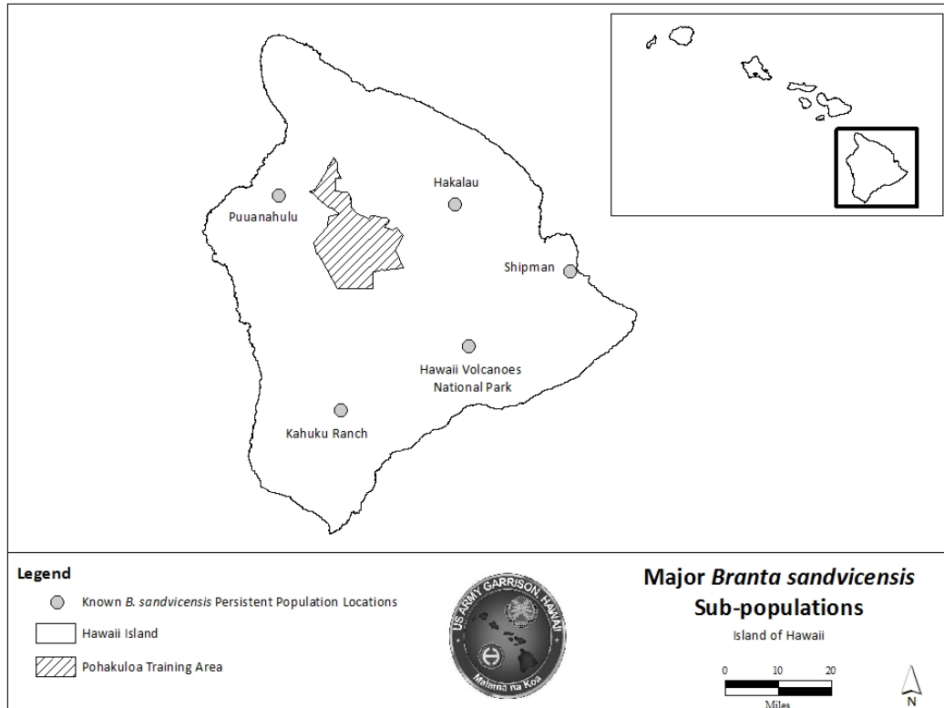
Figure 5. Spatial location of the five sub-populations of Hawaiian geese on the island of Hawaii in relation to Pohakuloa Training Area.
