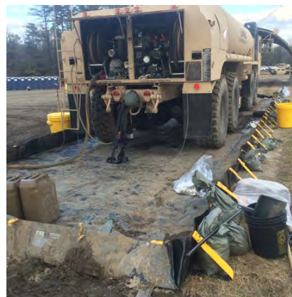
Mobile Secondary Containment
